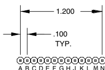
SINGLE POLE COMMON BUS TERMINAL
