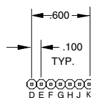
MATRIX TERMINAL PIN-OUT
