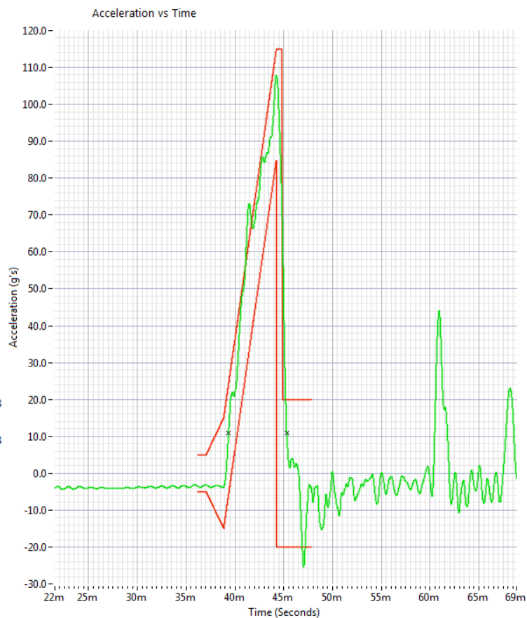
Figure 5 Mechanical Shock Half Sine Profile
