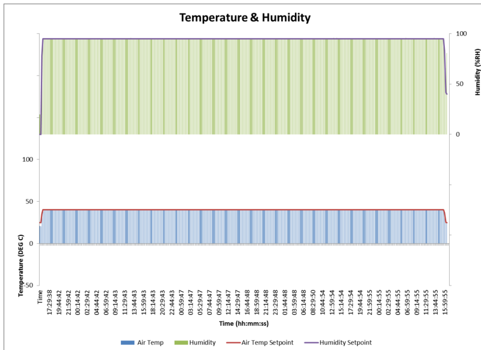
Figure 2 – Humidity Profile
