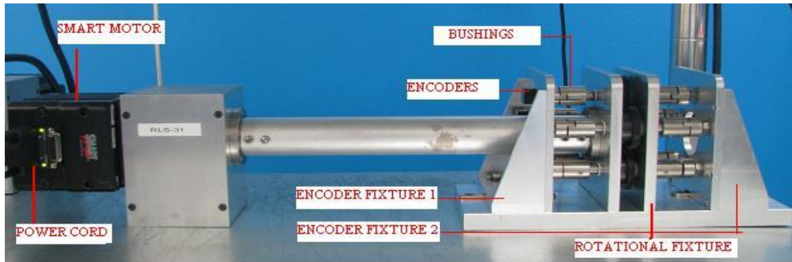
Figure 12 – Rotational Life Test Setup
